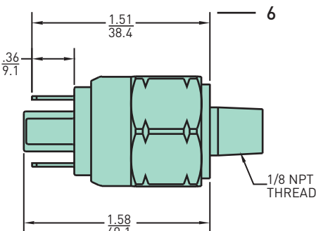
Pressure Switch
