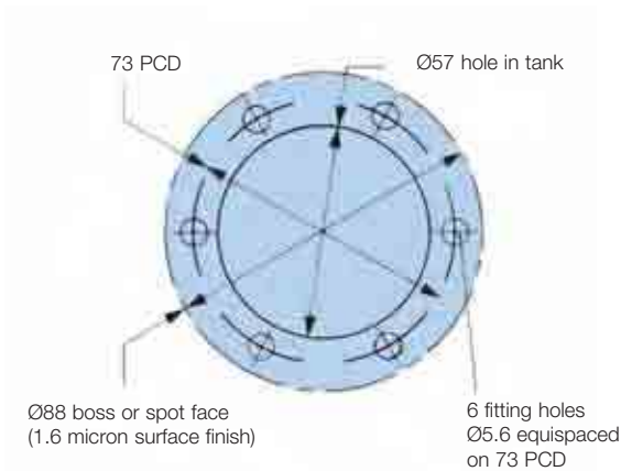
Mounting face for standard and large breather
